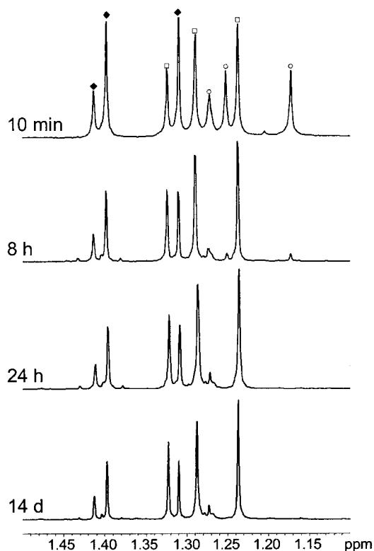
Figure 4. 500 MHz NMR spectra of the reaction of \text{Fe}_2(\text{S}_2\text{C}_3\text{H}_6)_2(\text{CO})_6 with 1 equiv of \text{Et}_4\text{NCN} in \text{CD}_3\text{CN} . Open circles (○) correspond to \text{Fe}_2(\text{S-}t\text{-Bu})_2(\text{CO})_6 , open squares (□) correspond to [\text{Fe}_2(\text{S-}t\text{-Bu})_2(\text{CN})_2(\text{CO})_5]^{2-} ( 6 ), and filled diamonds (◆) correspond to [\text{Fe}_2(\text{S-}t\text{-Bu})_2(\text{CN})_2(\text{CO})_4]^{2-} .
