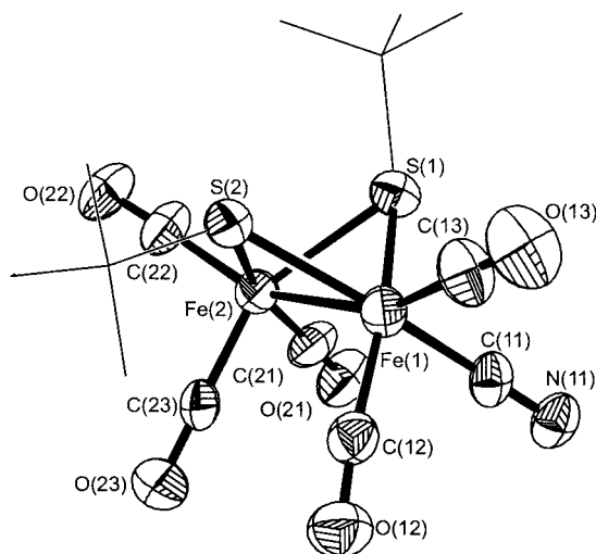
Figure 5. Structure of the major enantiomer of the anion in [K(18\text{-crown-6})][Fe_2(S\text{-}t\text{-Bu})_2(CN)(CO)_5] ( 6c ) with the thermal ellipsoids set at the 50% probability level. Selected distances (Å) and angles (deg): Fe(1)–Fe(2), 2.506(2); Fe(1)–C(11), 1.912(6); Fe(1)–C(12), 1.736(7); Fe(1)–C(13), 1.735(7); Fe(2)–C(21), 1.730(6); Fe(2)–C(22), 1.777(6); Fe(2)–C(23), 1.728(7); Fe(1)–S(1), 2.290(2); Fe(1)–S(2), 2.251(2); Fe(2)–S(1), 2.285(2); Fe(2)–S(2), 2.264(2); S(1)–Fe(1)–S(2), 79.18(7); S(1)–Fe(2)–S(2), 79.03(8).
