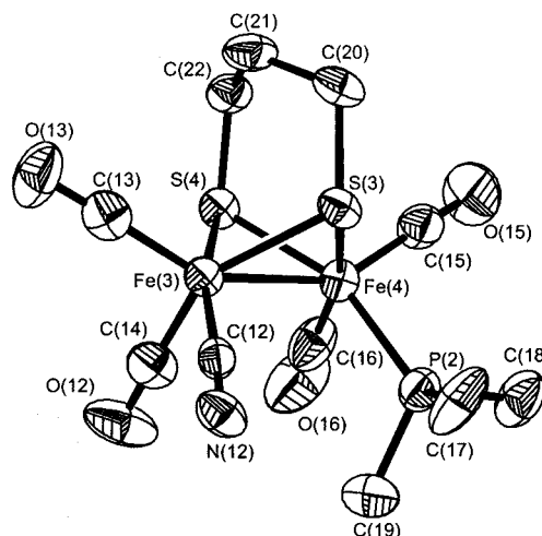
Figure 6. Structure of the anions in (Et_4N)[Fe_2(S_2C_3H_6)(CN)(CO)_4(PMe_3)]^- ( 7 ) with the thermal ellipsoids set at the 50% probability level. Selected distances (Å) and angles (deg): (Top) Fe(1)–Fe(2), 2.5365(11); Fe(1)–C(1), 1.919(6); Fe(1)–C(2), 1.742(6); Fe(1)–C(3), 1.741(6); Fe(2)–P(1), 2.2061(16); Fe(2)–C(4), 1.734(6); Fe(2)–C(5), 1.742(6); Fe(1)–S(1), 2.2708(15); Fe(1)–S(2), 2.2629(15); Fe(2)–S(1), 2.2740(15); Fe(2)–S(2), 2.2561(15); S(1)–Fe(1)–S(2), 85.25(5); S(1)–Fe(2)–S(2), 85.33(5). (Bottom) Fe(3)–Fe(4), 2.5593(11); Fe(3)–C(12), 1.920(6); Fe(3)–C(13), 1.766(6); Fe(3)–C(14), 1.747(6); Fe(4)–P(2), 2.2055(17); Fe(4)–C(15), 1.763(6); Fe(4)–C(16), 1.747(7); Fe(3)–S(3), 2.2727(15); Fe(3)–S(4), 2.2560(15); Fe(4)–S(3), 2.2635(15); Fe(4)–S(4), 2.2538(16); S(3)–Fe(3)–S(4), 84.67(5); S(3)–Fe(4)–S(4), 84.93(5).
