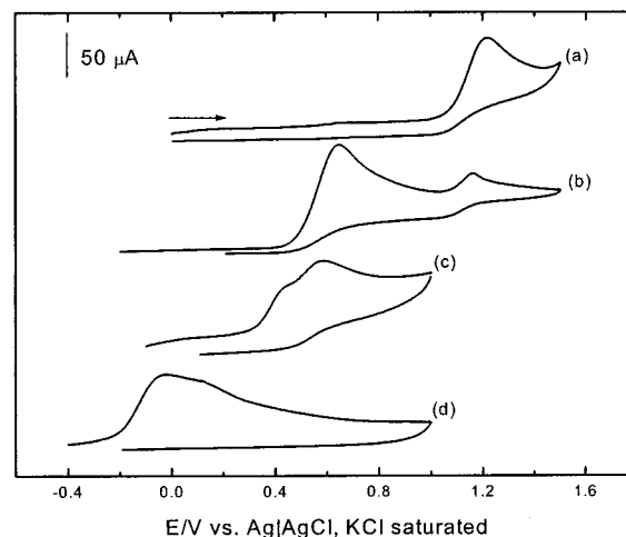
Figure 2. Voltammograms ( 200\text{ mV s}^{-1} ) of \text{Fe}_2(\text{S}_2\text{C}_3\text{H}_6)(\text{CO})_6 (a), \text{Fe}_2(\text{S}_2\text{C}_3\text{H}_6)(\text{CNMe})_2(\text{CO})_4 (b), (\text{Et}_4\text{N})[\text{Fe}_2(\text{S}_2\text{C}_3\text{H}_6)(\text{CN})(\text{CO})_5] (c), and (\text{Et}_4\text{N})_2[\text{Fe}_2(\text{S}_2\text{C}_3\text{H}_6)(\text{CN})_2(\text{CO})_4] (d) in \text{MeCN}-\text{Bu}_4\text{NPF}_6 at a glassy carbon electrode. Anodic currents are positive.
